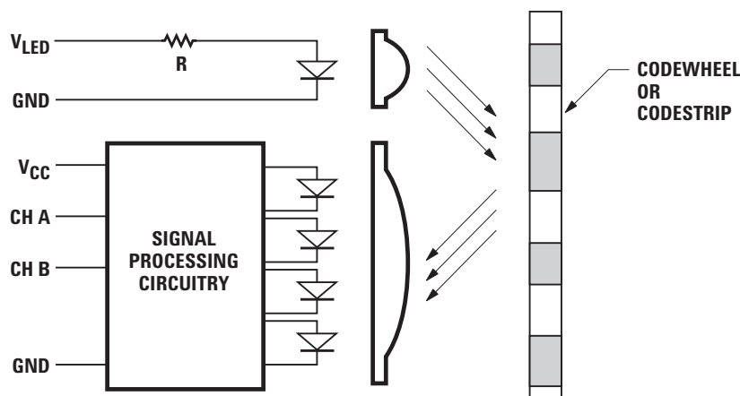
Figure 1. Block Diagram of AEDR-8300.
