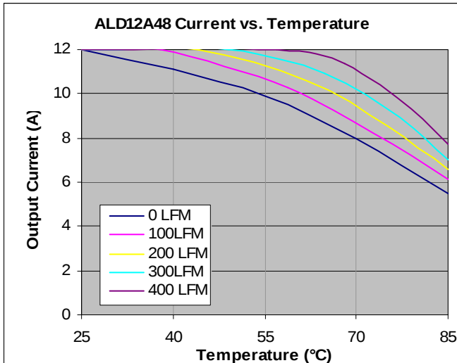
Figure 10. 5V Output current vs. ambient temperature curves at V_{IN} = 48Vdc .
