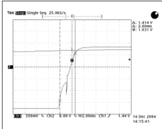
Figure 26. 1.8V Startup Characteristic at V_{IN} = 36Vdc , I_O = \text{Full Load} , T_A = 25^\circ C , C_O = 0 .
