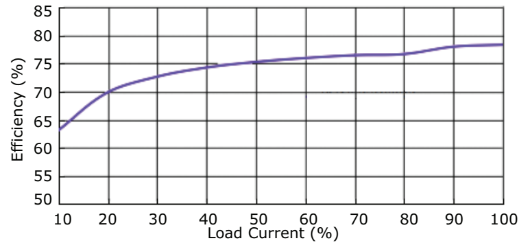
AE10-EW-S9 Efficiency Curve Efficiency vs. Load Current
