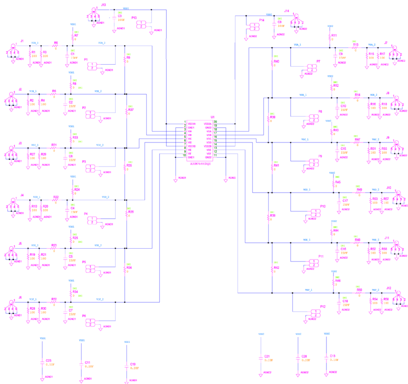
Figure 4. EVAL-ADuM7643EBZ Schematic
