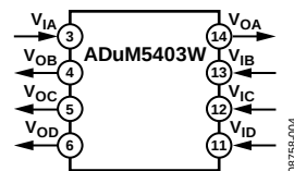
Figure 4. ADuM5403W
