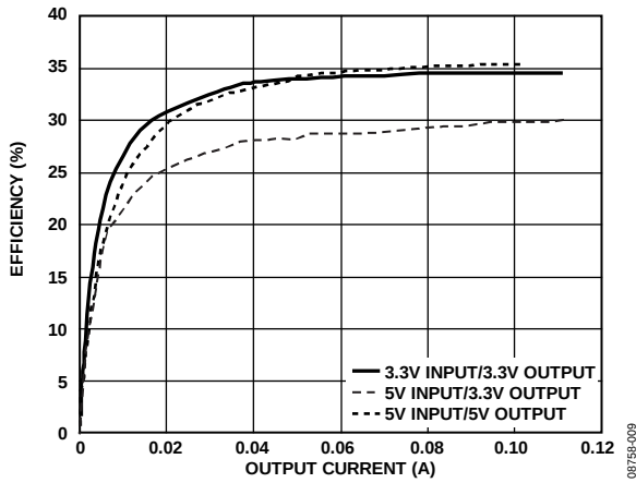
Figure 9. Typical Power Supply Efficiency at 5 V Input/5 V Output and 3.3 V Input/3.3 V Output
