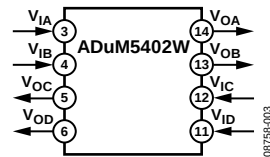
Figure 3. ADuM5402W
