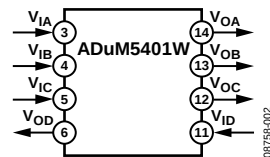
Figure 2. ADuM5401W
