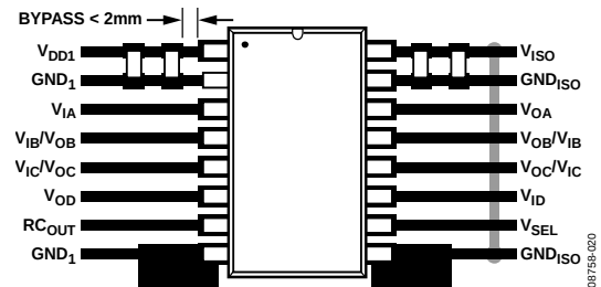
Figure 23. Recommended Printed Circuit Board Layout
