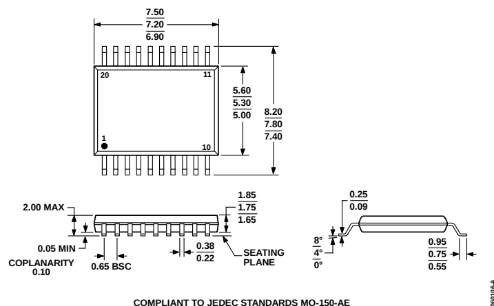
Figure 22. 20-Lead Shrink Small Outline Package [SSOP] (RS-20) Dimensions shown in millimeters
