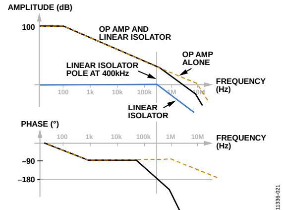
Figure 30. Bode Plot 1: Op Amp and Linear Isolator
