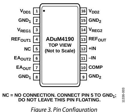
Figure 3. Pin Configuration
