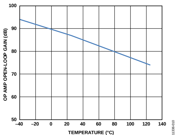
Figure 10. Op Amp Open-Loop Gain vs. Temperature
