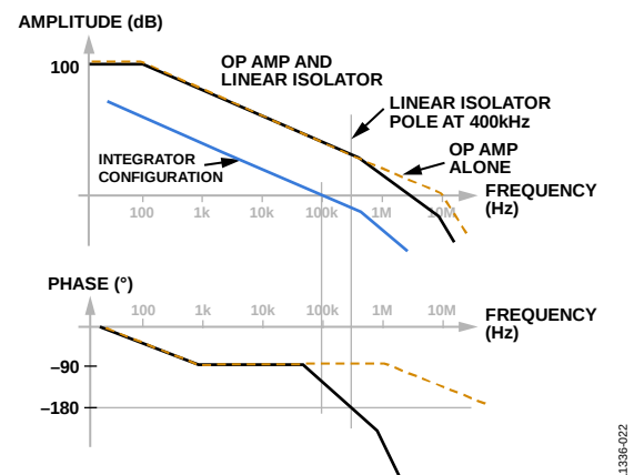
Figure 31. Bode Plot 2: Op Amp and Linear Isolator with Integrator Configuration
