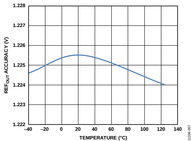
Figure 7. \text{REF}_{OUT} Accuracy vs. Temperature
