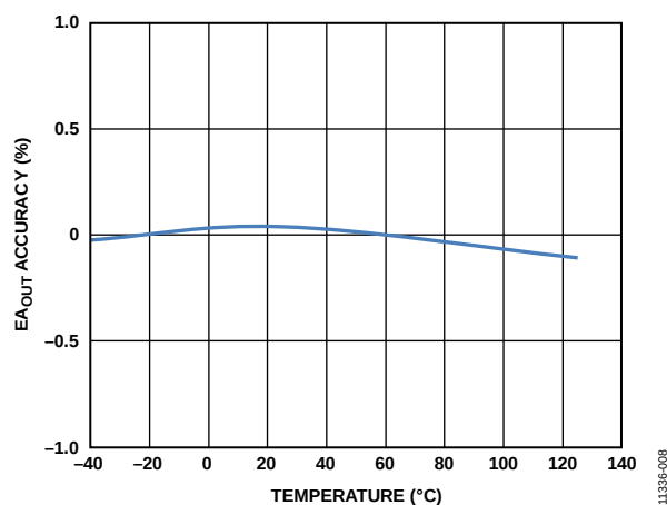
Figure 8. \text{EA}_{OUT} Accuracy vs. Temperature
