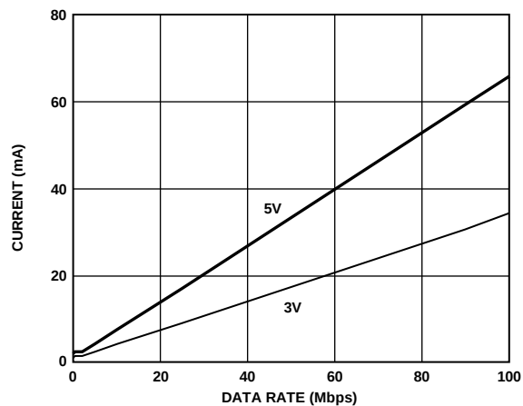
Figure 13. Typical ADuM3401-EP V_{DD1} Supply Current vs. Data Rate for 5V and 3.3V Operation
