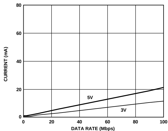
Figure 12. Typical ADuM3400-EP V_{DD2} Supply Current vs. Data Rate for 5V and 3.3V Operation
