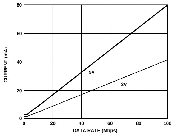
Figure 11. Typical ADuM3400-EP V_{DD1} Supply Current vs. Data Rate for 5V and 3.3V Operation
