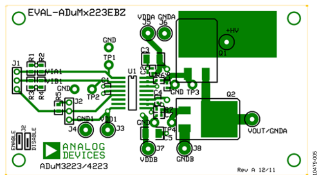
Figure 5. Top Layer
