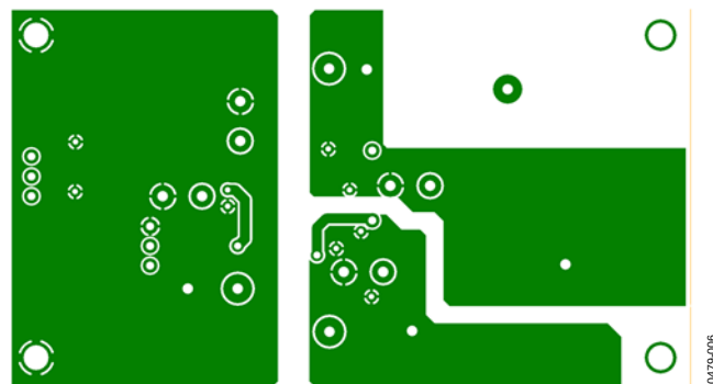
Figure 6. Bottom Layer
