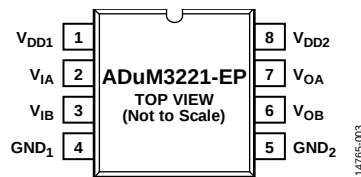
Figure 3. Pin Configuration
