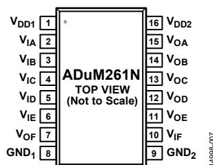
Figure 7. ADuM261N Pin Configuration
