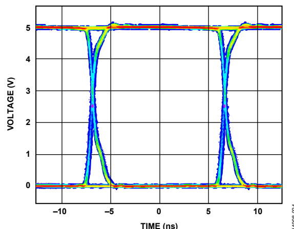
Figure 24. ADuM260N/ADuM261N/ADuM262N/ADuM263N Eye Diagram
