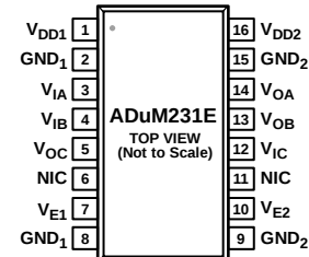
Figure 9. ADuM231E Pin Configuration
