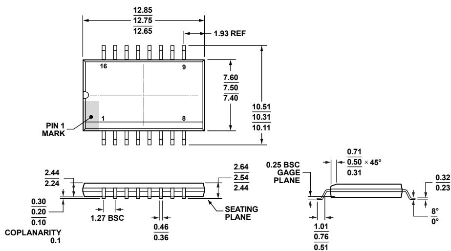
Figure 13. 16-Lead Standard Small Outline Package, with Increased Creepage [SOIC_IC]
