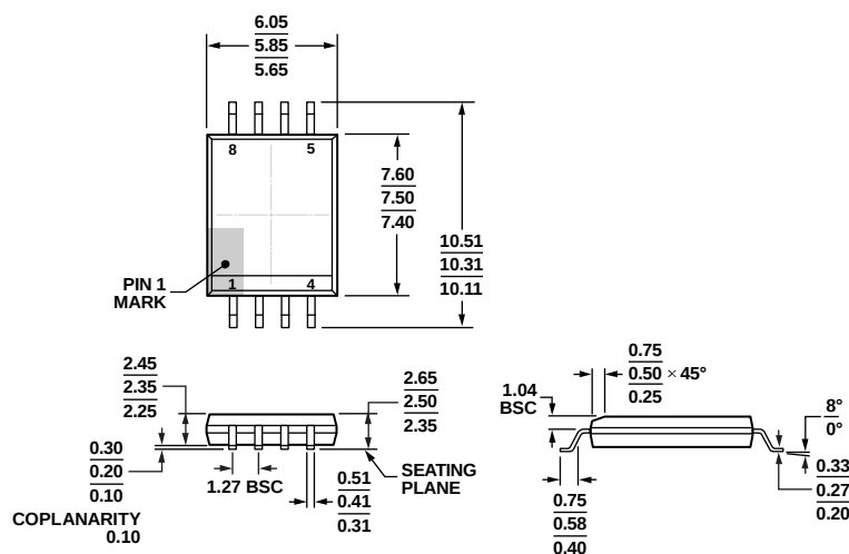
Figure 24. 8-Lead Standard Small Outline Package, with Increased Creepage [SOIC_IC] Wide Body (RI-8-1)
