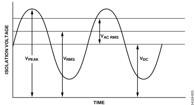
Figure 23. Critical Voltage Example
