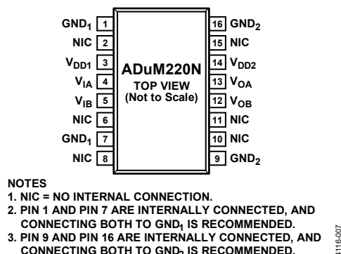
Figure 7. ADuM220N Pin Configuration
