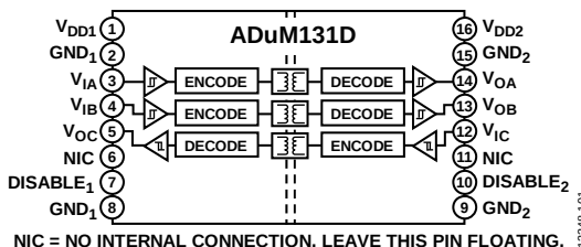
Figure 3. ADuM131D Functional Block Diagram
