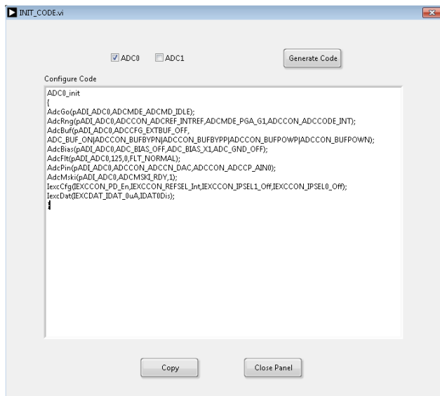
Figure 22. Generate Code Window
