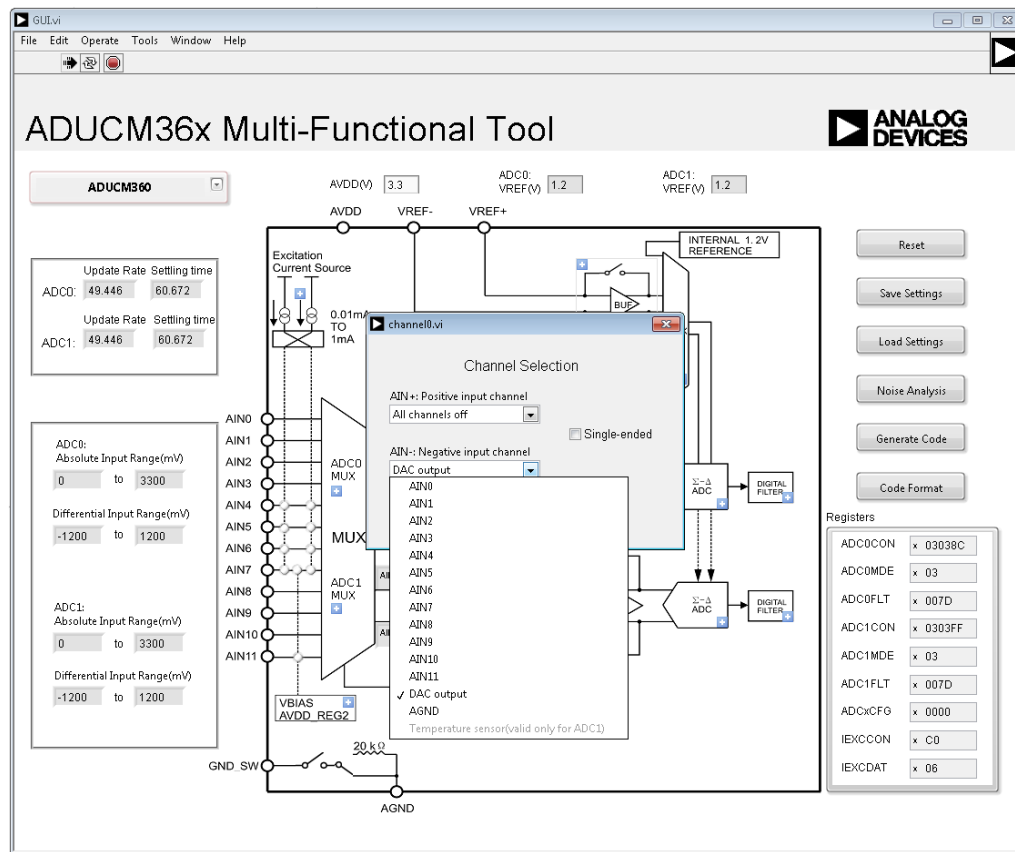
Figure 12. Input Channels Selection
