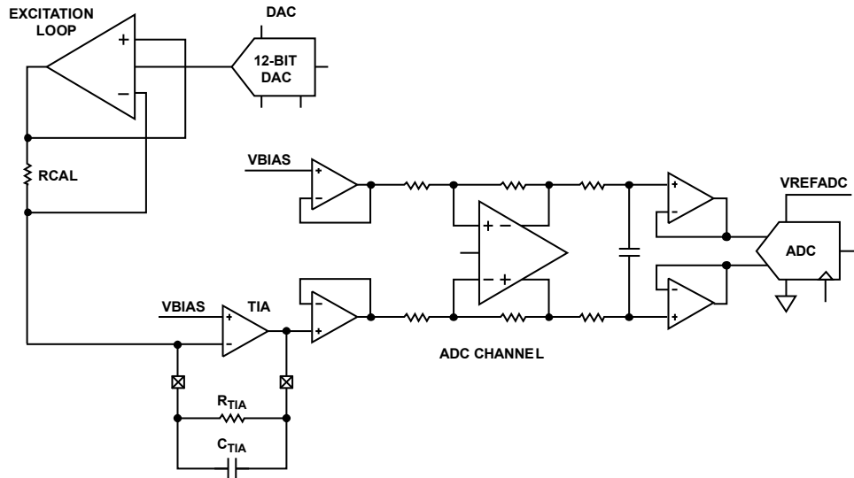
Figure 129. Calibrate R_{\text{GAIN}} , Simplified Diagram
