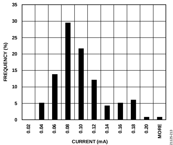
Figure 16. Sleep Mode Current Distribution at 3.0 V Supply
