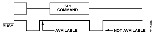
Figure 37. Busy Signal ( \overline{\text{BUSY}} ) Orientation After SPI Command
