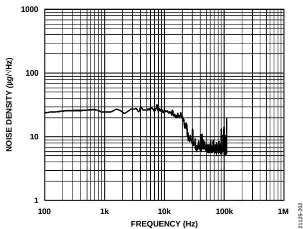
Figure 7. Noise Density, Wideband, MTC, AVG_CNT = 0
