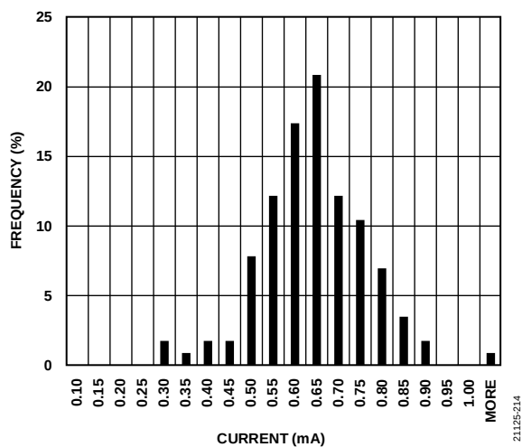
Figure 17. Sleep Mode Current Distribution at 3.3 V Supply
