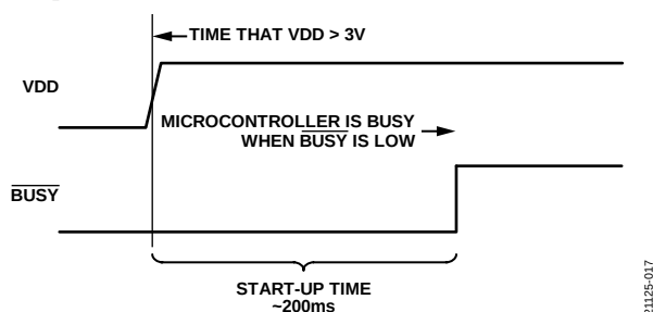
Figure 38. \overline{\text{BUSY}} Response During Start Up
