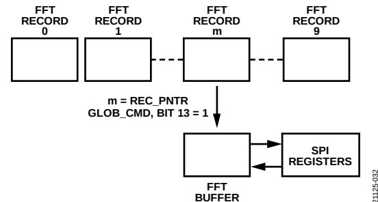
Figure 31. FFT Record Access
