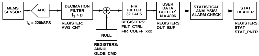
Figure 40. MTC Mode Datapath Processing
