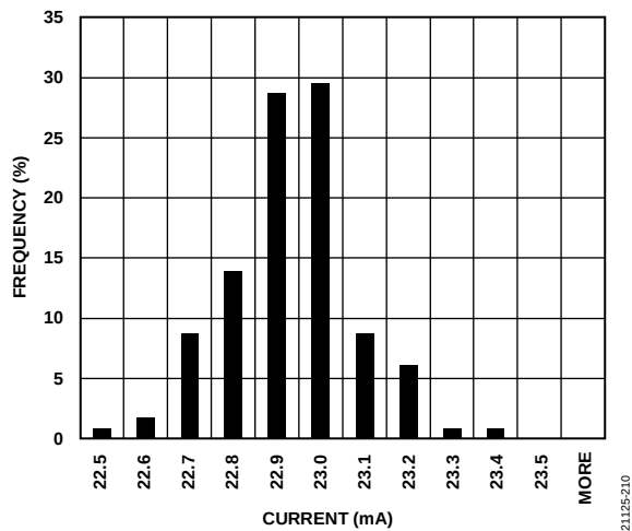
Figure 13. Operating Mode Current Distribution at 3.0 V Supply
