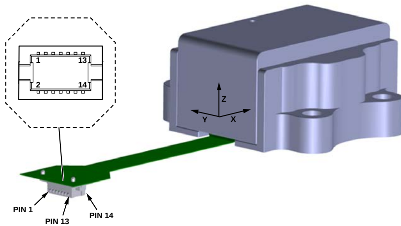
Figure 6. Pin Configuration
