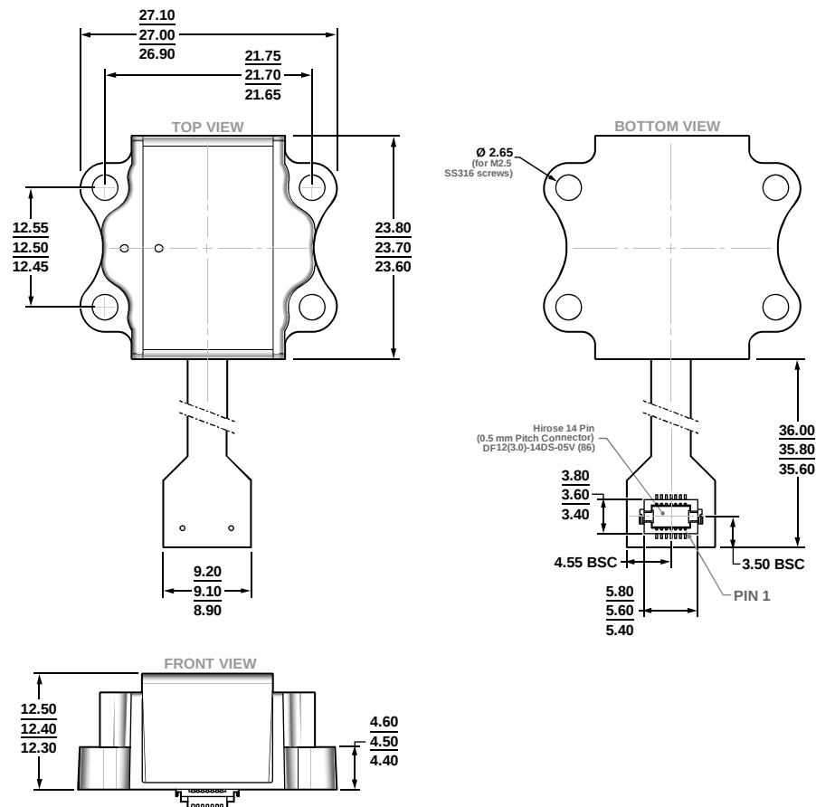
Figure 45. 14-Lead Module with Integrated Flex Connector [MODULE] (ML-14-7)
