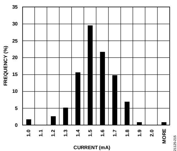
Figure 18. Sleep Mode Current Distribution at 3.6 V Supply
