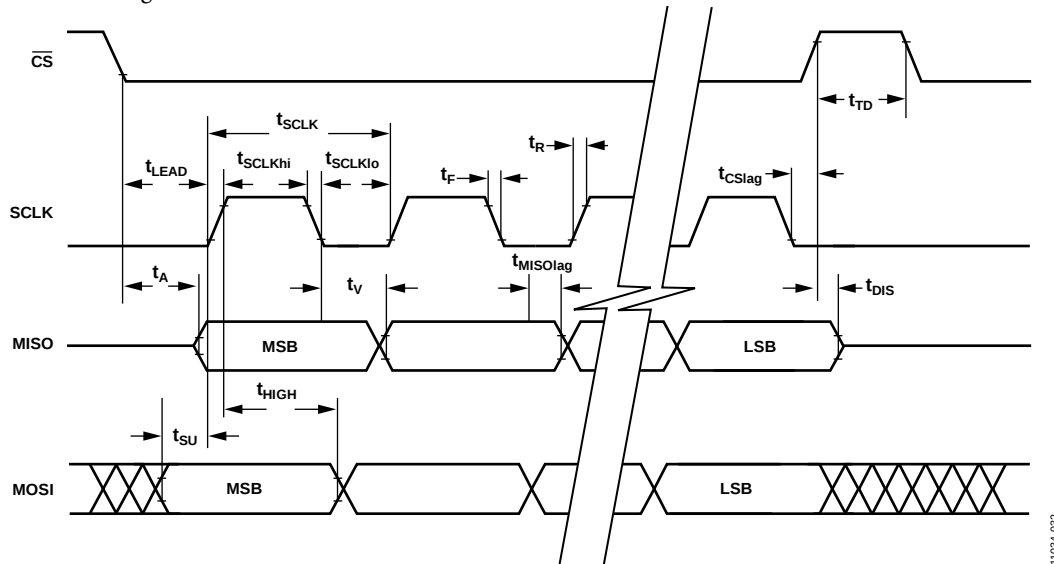
Figure 18. SPI Timings Drawing
