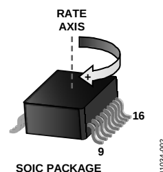
Figure 2. RATEOUT Signal Increases with Clockwise Rotation
