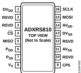
Figure 3. Pin Configuration
