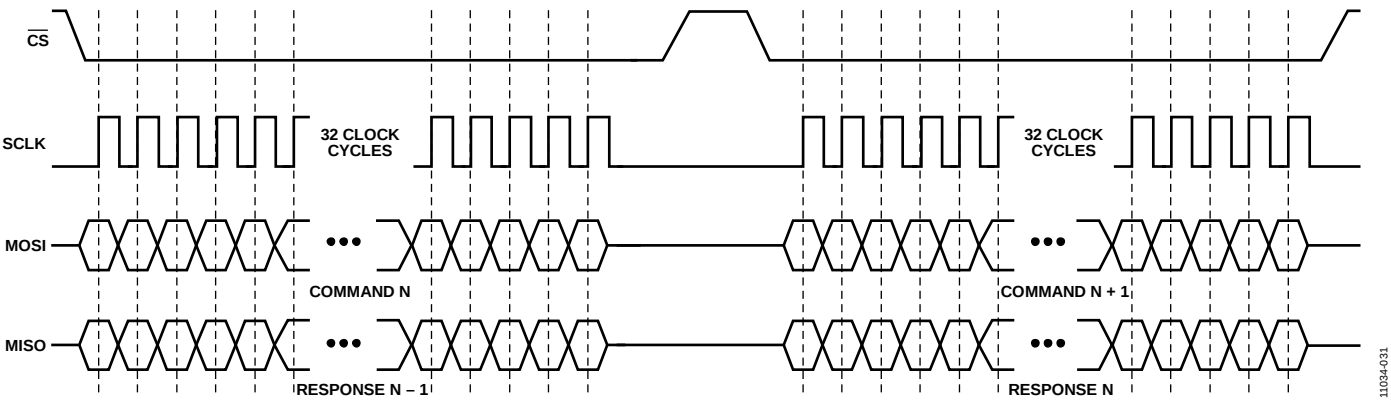
Figure 20. SPI Protocol
