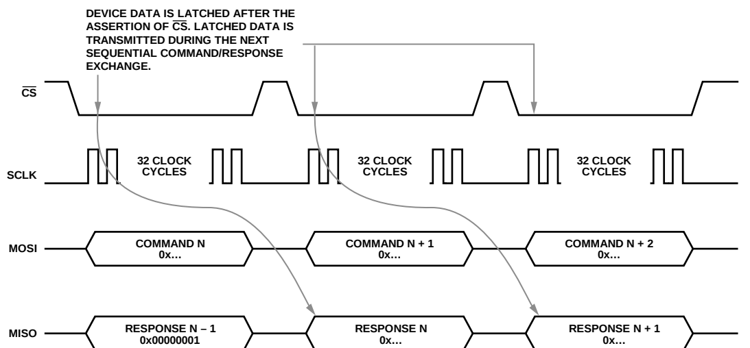
Figure 19. Device Data Latching
