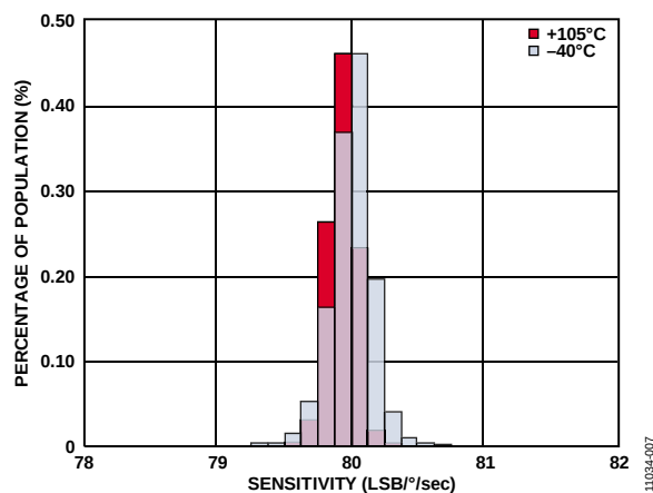
Figure 7. Sensitivity
