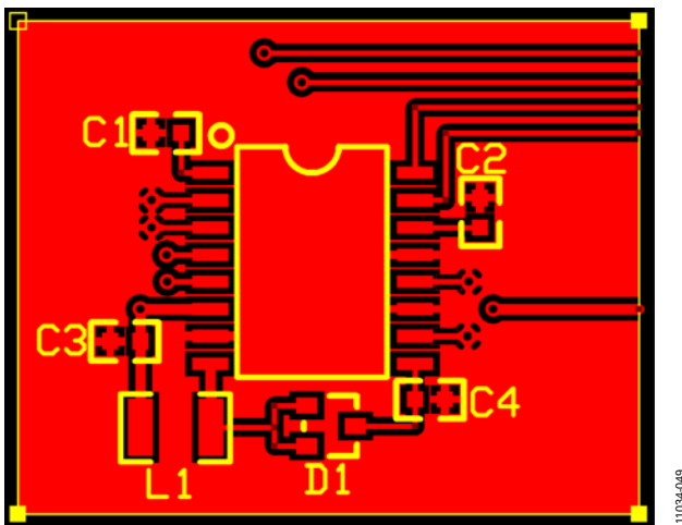
Figure 22. SOIC PCB Layout Top Layer Metal
