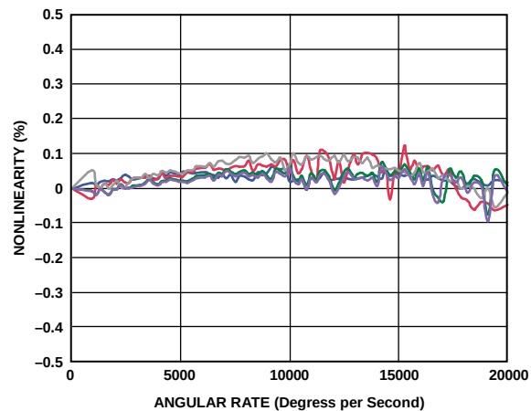
Figure 17. Typical Nonlinearity (Four Typical Devices)
