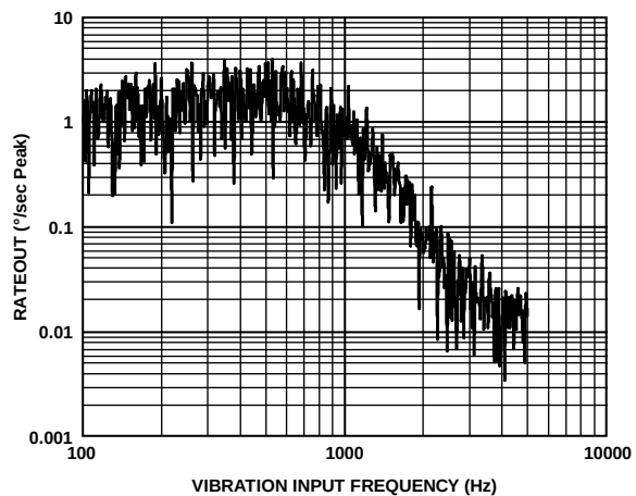
Figure 16. Typical Response to 10 g RMS Sinusoidal Vibration (Sensor Bandwidth = 1 kHz)
