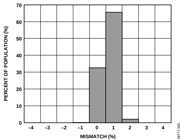
Figure 12. Self-Test Mismatch at 25°C ( V_{RATIO} = 5\text{ V} )
