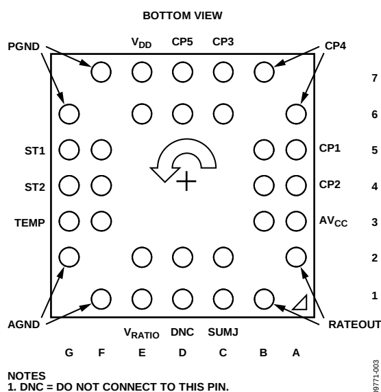
Figure 3. Pin Configuration
