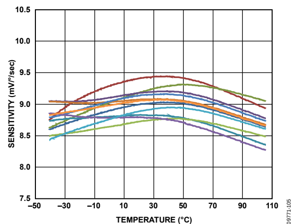
Figure 8. Sensitivity over Temperature, 16 Parts in Sockets
