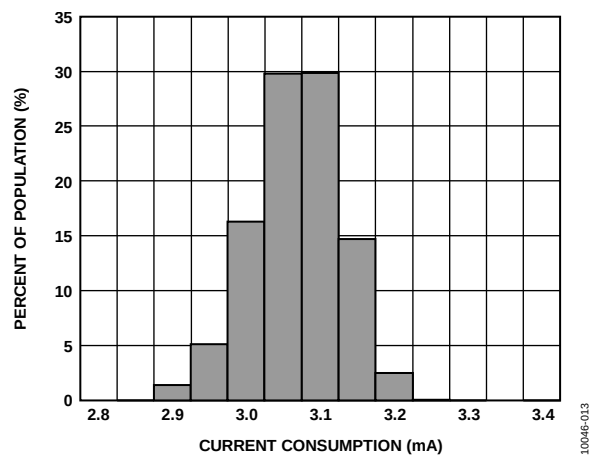
Figure 18. Current Consumption at 25°C ( V_{RATIO} = 5 V)
