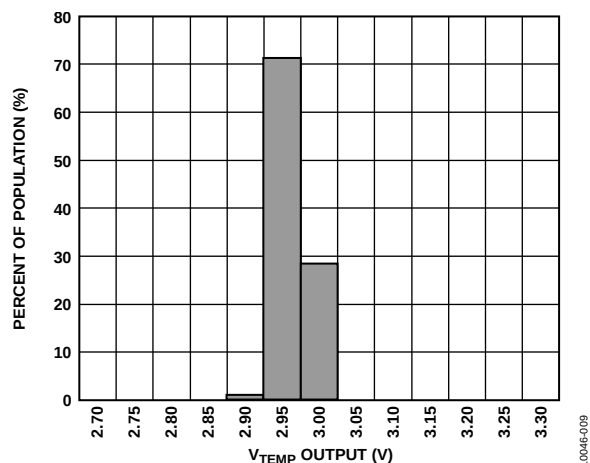
Figure 16. V_{TEMP} Output at 25°C ( V_{RATIO} = 5 V)
