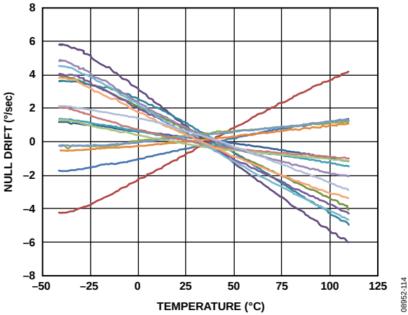
Figure 13. Null Drift over Temperature
