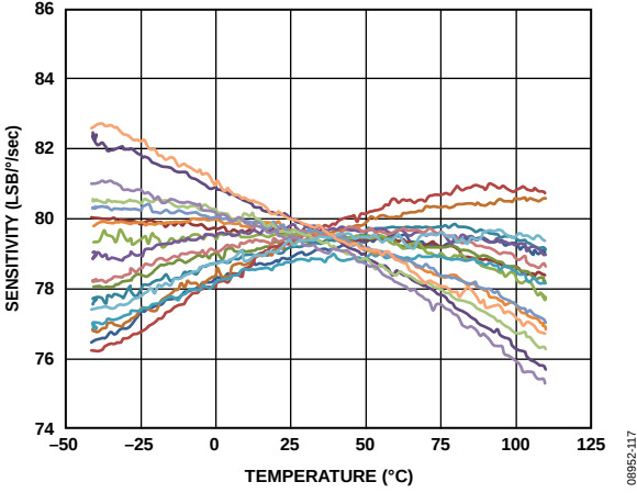
Figure 15. Sensitivity over Temperature
