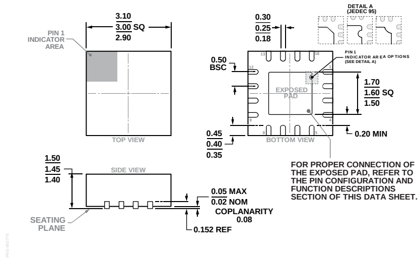
Figure 18. 16-Lead Lead Frame Chip Scale Package [LFCSP] 3 mm × 3 mm Body and 1.45 mm Package Height (CP-16-28) Dimensions shown in millimeters
