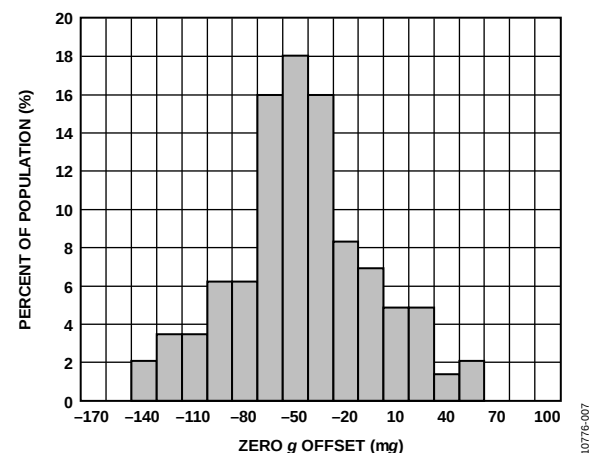
Figure 7. Z-Axis Zero g Offset at 25°C, V_S = 2\text{ V}
