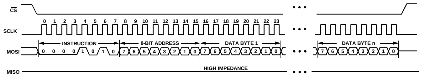
Figure 39. Burst Write
