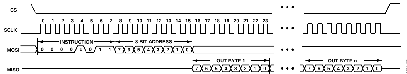
Figure 38. Burst Read
