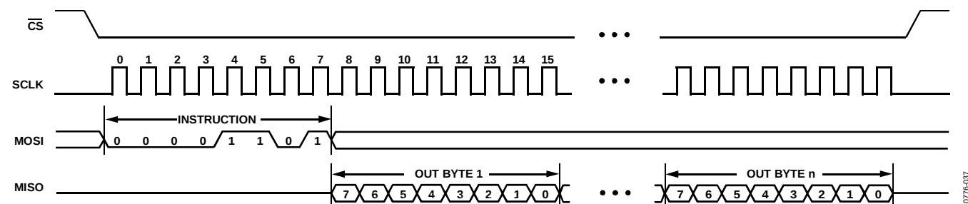
Figure 40. FIFO Read
