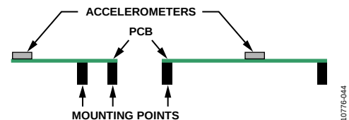
Figure 49. Incorrectly Placed Accelerometers
