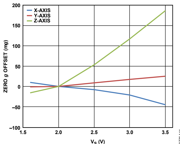
Figure 49. 0 g Offset vs. Supply Voltage
