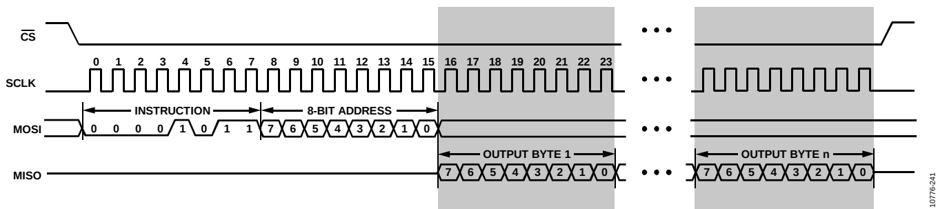
Figure 38. Burst Read
