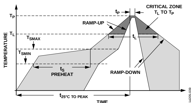
Figure 75. Recommended Soldering Profile
