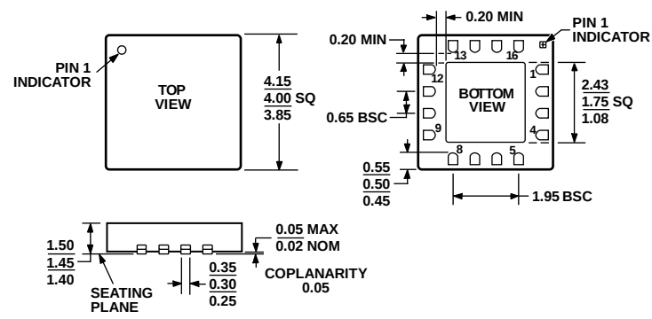
Figure 33. 16-Lead Lead Frame Chip Scale Package [LFCSP_LQ] 4 mm × 4 mm Body, Thick Quad (CP-16-5a*) Dimensions shown in millimeters
