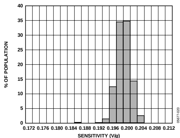
Figure 22. Z-Axis Sensitivity at 25°C, V_S = 2\text{ V}
