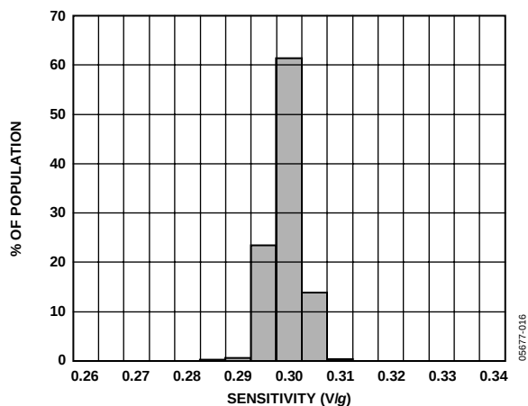
Figure 18. Y-Axis Sensitivity at 25°C, V_S = 3\text{ V}
