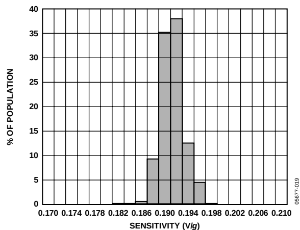
Figure 21. Y-Axis Sensitivity at 25°C, V_S = 2\text{ V}
