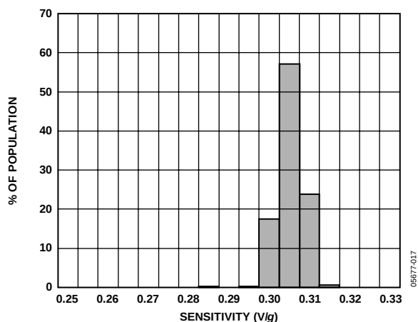
Figure 19. Z-Axis Sensitivity at 25°C, V_S = 3\text{ V}
