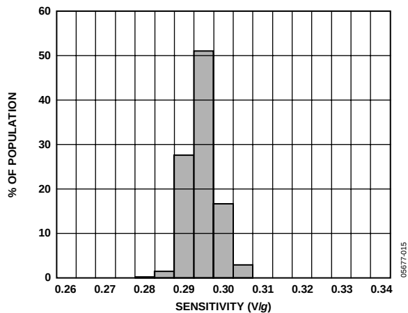
Figure 17. X-Axis Sensitivity at 25°C, V_S = 3\text{ V}
