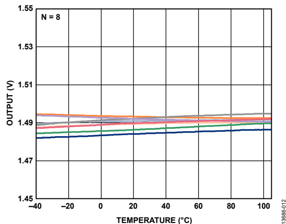
Figure 12. X-Axis Zero g Bias vs. Temperature
