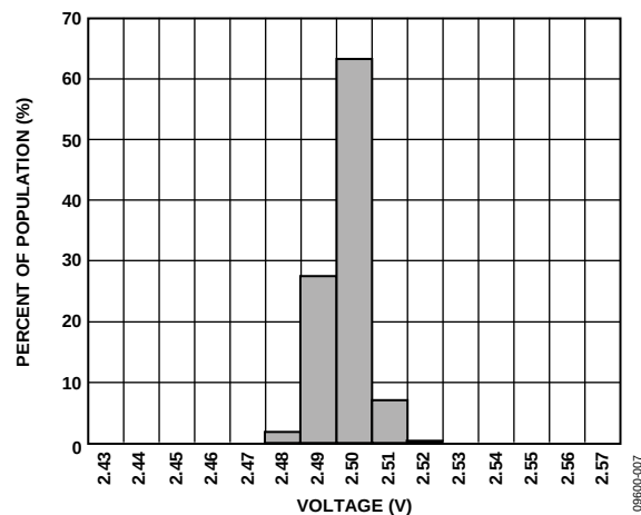
Figure 7. Y-Axis Zero g Bias at T_A = 25^\circ\text{C}
