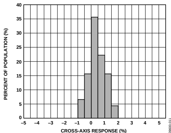
Figure 13. Cross-Axis Response, Z-Axis vs. Y-Axis
