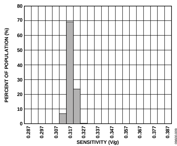
Figure 9. Y-Axis Sensitivity at T_A = 25^\circ\text{C}
