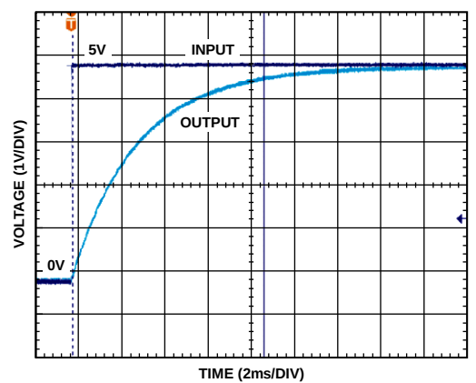
Figure 15. Turn-On Time, C_x, C_y = 0.1 \mu F , Time Scale = 2 ms/div
