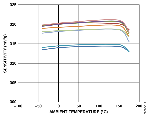
Figure 14. Y-Axis Sensitivity over Temperature, Nine Devices
