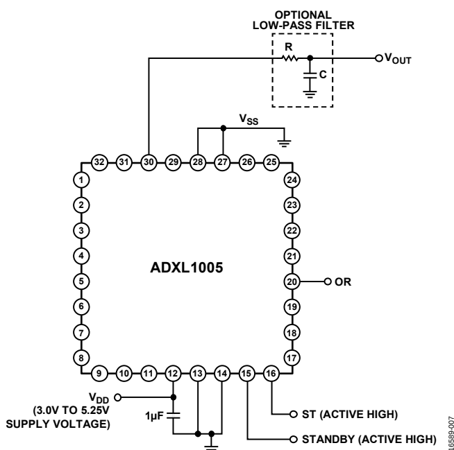
Figure 20. Application Circuit
