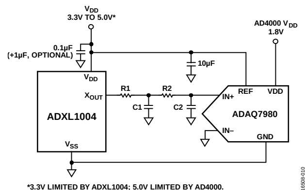
Figure 23. Application Circuit for the ADXL1004
