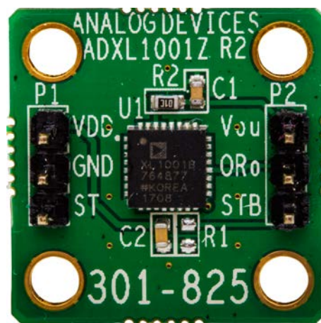
Figure 1. EVAL-ADXL1001Z
