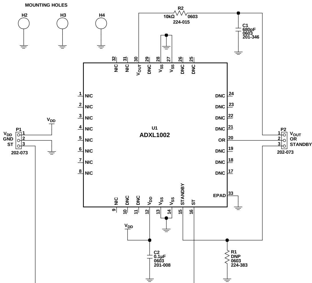
Figure 4. EVAL-ADXL100Z Schematic
