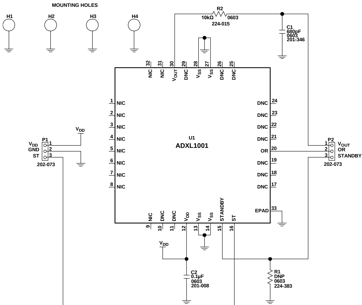
Figure 3. EVAL-ADXL1001Z Schematic
