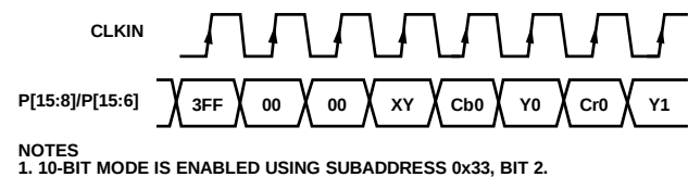
Figure 61. ED (at 54 MHz) Input Sequence (EAV/SAV)
