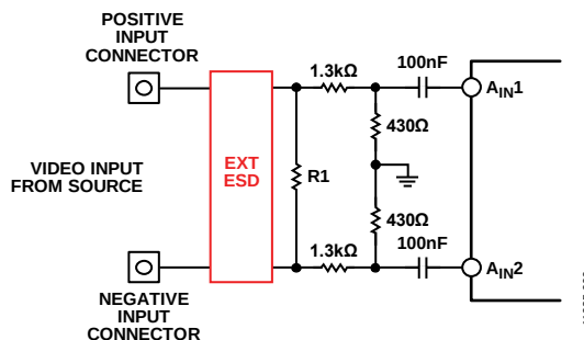
Figure 10. Differential Input Network
