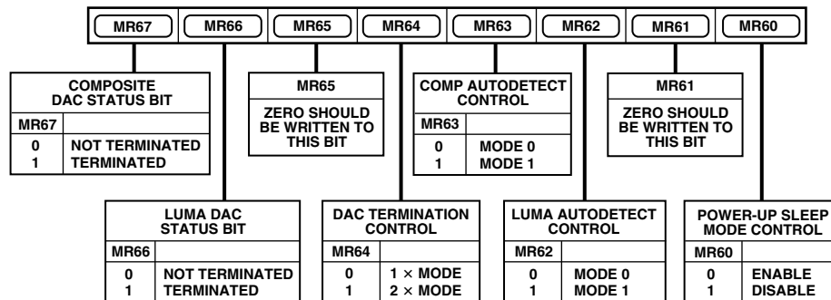
Figure 50. Mode Register 6 (MR6)
