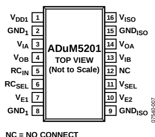
Figure 7. ADuM5201 Pin Configuration
