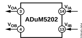
Figure 4. ADuM5202
