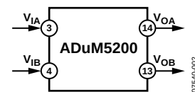
Figure 2. ADuM5200
