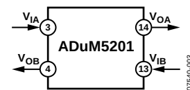
Figure 3. ADuM5201
