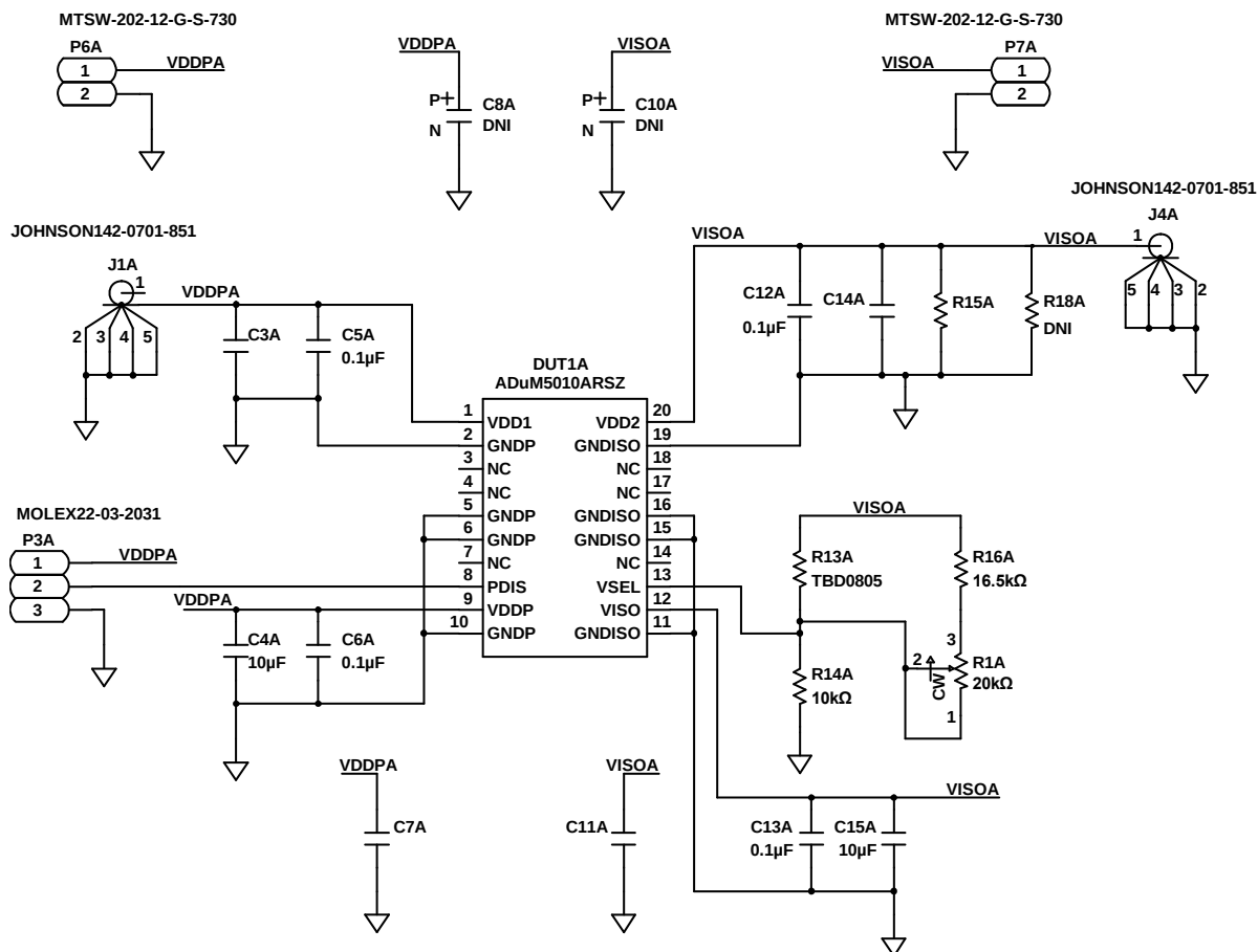
Figure 3. ADuM5010/ADuM6010 Schematic
