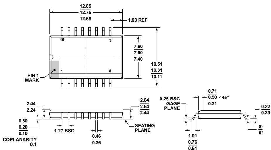
Figure 30. 16-Lead Standard Small Outline Package, with Increased Creepage [SOIC_IC] Wide Body (RI-16-2) Dimensions shown in millimeters
