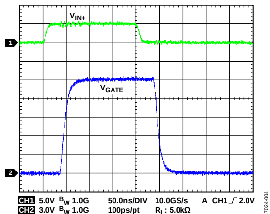
Figure 4. V_{IN+} to V_{GATE} Waveform, V_{DD1} = 5V , V_{DD2} = 15V , 10\Omega Gate Resistors, 2nF Load, SRC Low
