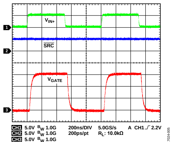
Figure 5. V_{IN+} to V_{GATE} Waveform, V_{DD1} = 5V , V_{DD2} = 15V , 10\Omega Gate Resistors, 2nF Load, Both Edges Slow
