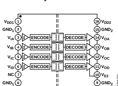
Figure 1. ADuM1400
