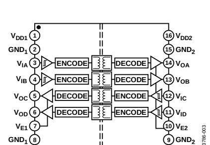
Figure 3. ADuM1402
