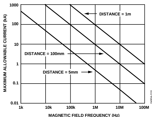
Figure 16. Maximum Allowable Current for Various Current-to-ADuM131x Spacings
