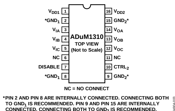
Figure 4. ADuM1310 Pin Configuration
