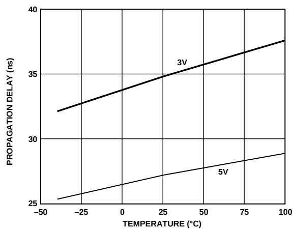
Figure 13. Propagation Delay vs. Temperature, C Grade
