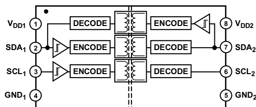
图2. ADuM1251
