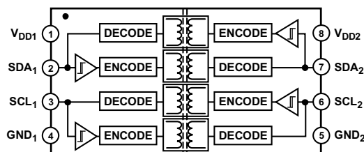
图1. ADuM1250
