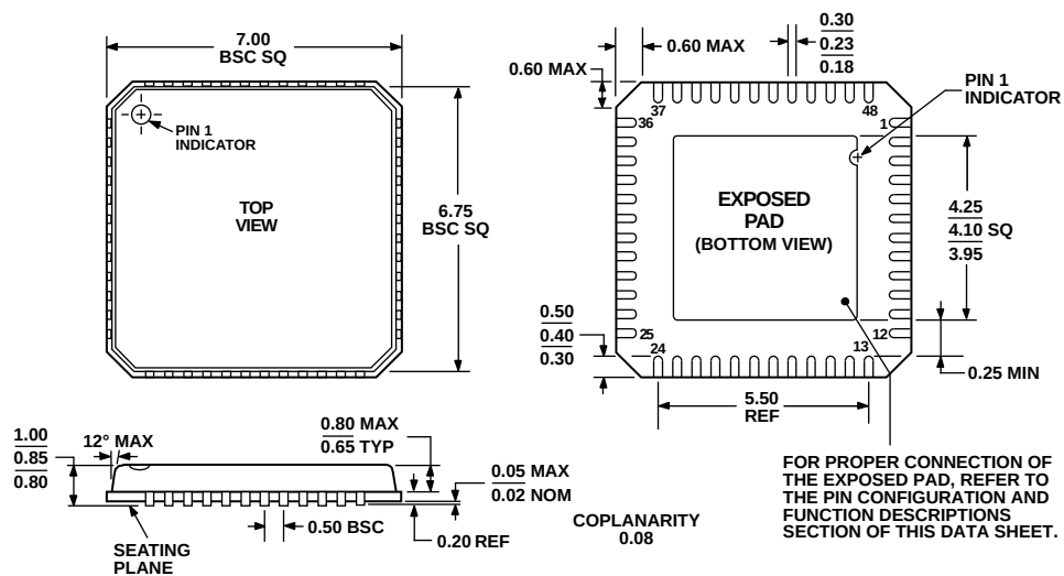
Figure 31. 48-Lead Lead Frame Chip Scale Package [LFCSP_VQ] 7 mm x 7 mm Body, Very Thin Quad (CP-48-3)
