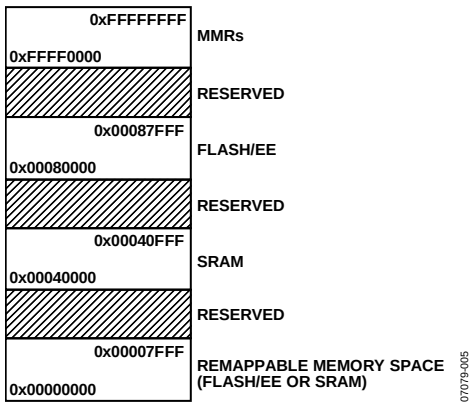
Figure 10. Memory Map
