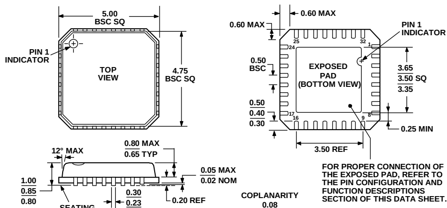
Figure 30. 32-Lead Lead Frame Chip Scale Package [LFCSP_VQ] 5 mm x 5 mm Body, Very Thin Quad (CP-32-4)
