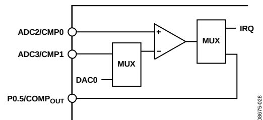
Figure 34. Comparator
