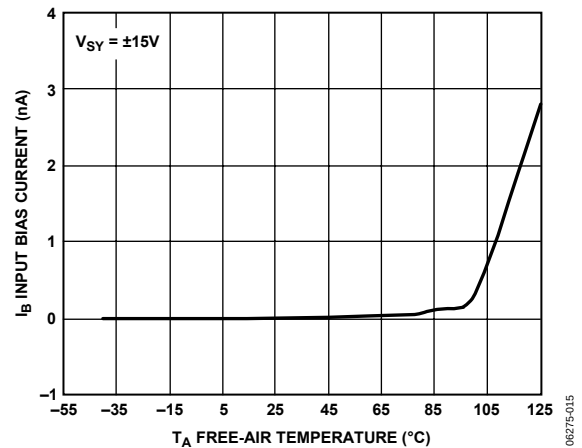
Figure 15. Input Bias Current vs. Free-Air Temperature
