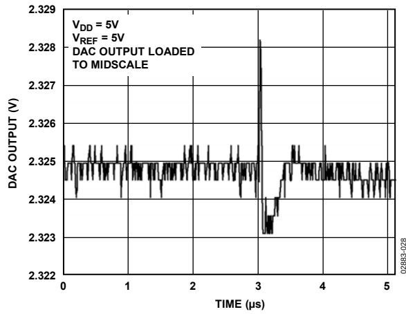
Figure 27. DAC-to-DAC Crosstalk
