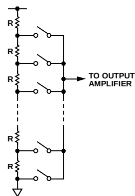
Figure 43. Resistor String
