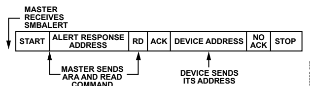
Figure 68. INT/ \overline{\text{INT}} Responds to SMBALERT ARA
